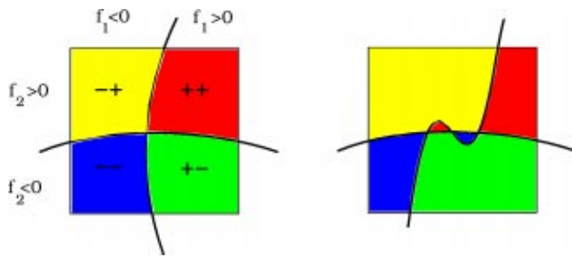
FIG. 1. (Color online) Sketch of the domains where f_1, f_2 have the indicated combination of signs.
