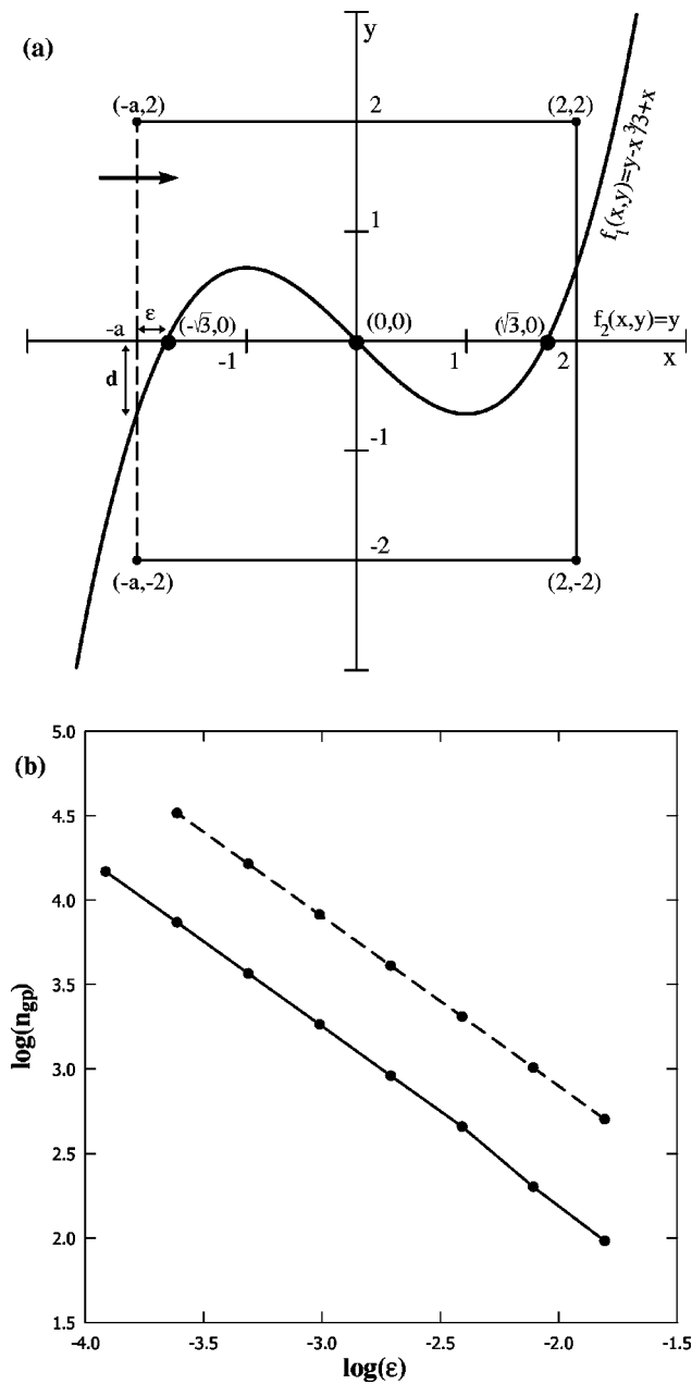
FIG. 8. (a) Plot of the curves f_1 \equiv y - \frac{1}{3}x^3 + x = 0 and f_2 \equiv y = 0 . (b) Number of iteration points n_{gp} used to compute the correct value of the TD on a domain for the set of equation of panel (a) (dashed line) and the SM (continuous line), versus the distance \epsilon of a root from the boundary of the domain.
