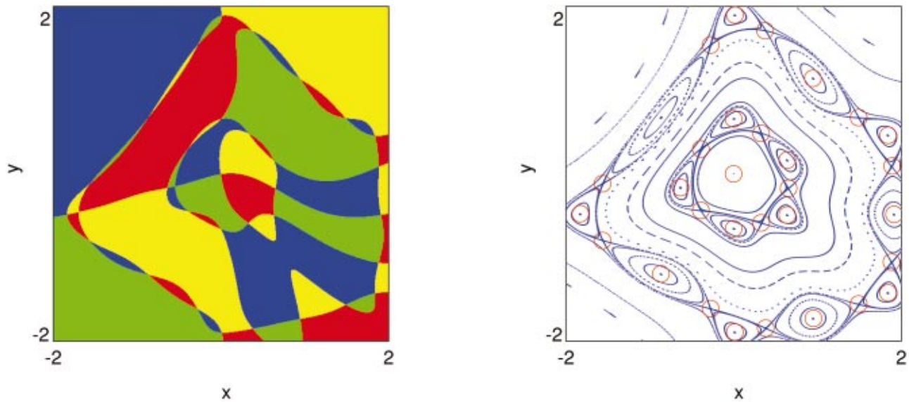
FIG. 2. (Color) Beam-beam map for \omega=0.21 : color map , for p=5 iterations of the map, computed on a square lattice of 2^n \times 2^n points with n=9 (left); phase plot of the map (right): the red circles denote the position of the fixed points found with initial guesses taken in boxes of size m\epsilon with \epsilon=2^{-n} and m=7 .
